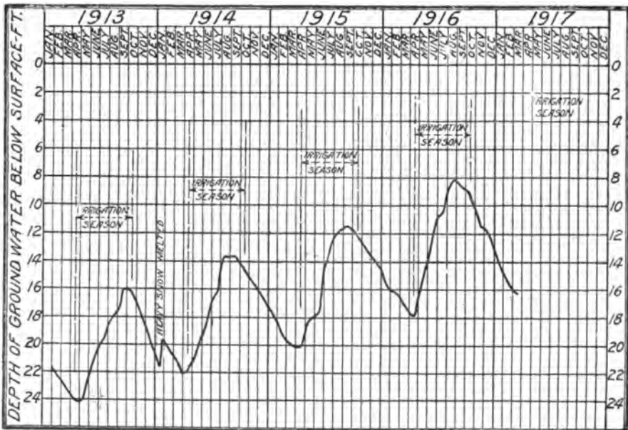
FIG. 59.—Curve Showing the Seasonal Fluctuation and Rise of Ground Water in Boise Valley, Idaho. After Burkholder.
